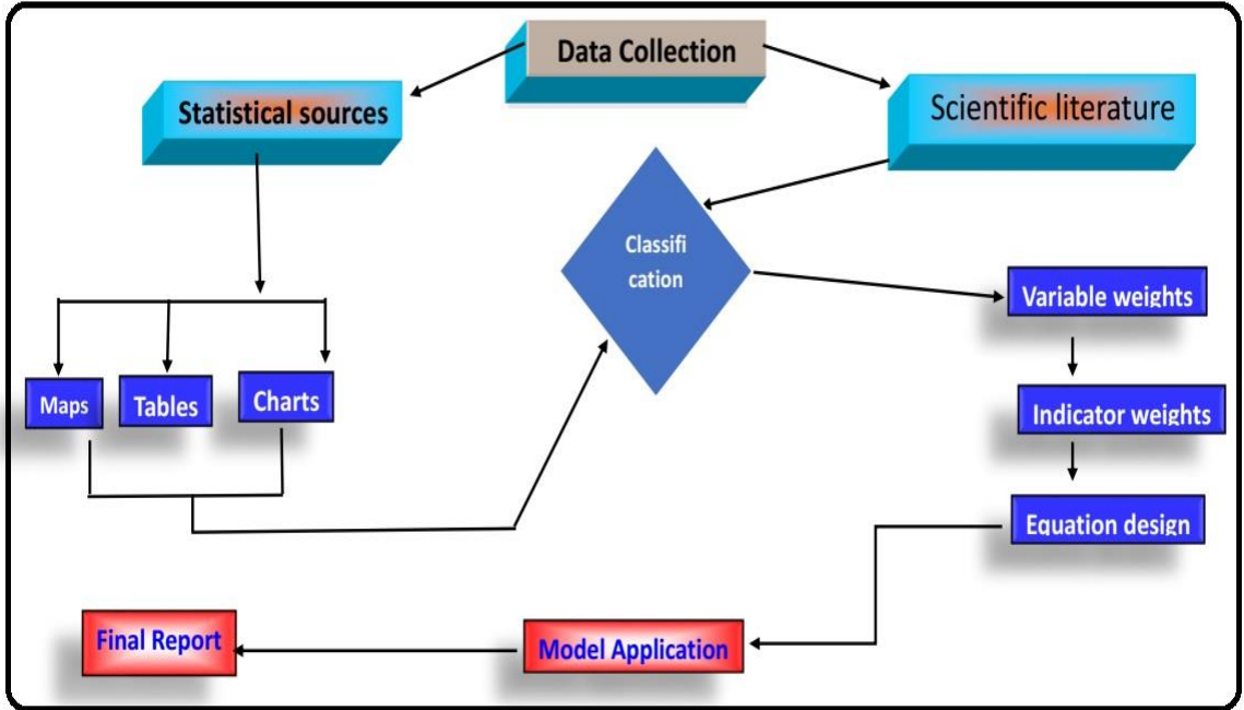
Figure 3: Model methodology
